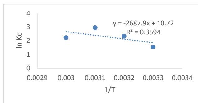
Fig 7. Van't Hoff plot for adsorption of CR onto AC-CPH
