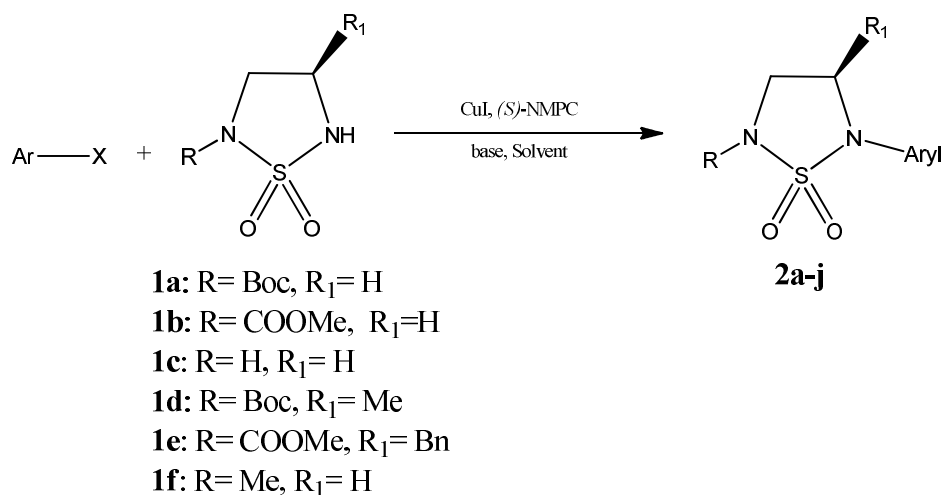
Scheme 1. Synthetic route for Copper-(S)-NMP-catalyzed N -arylation of N 5 H -1,2,5-thiadiazolidine 1,1-dioxides.
