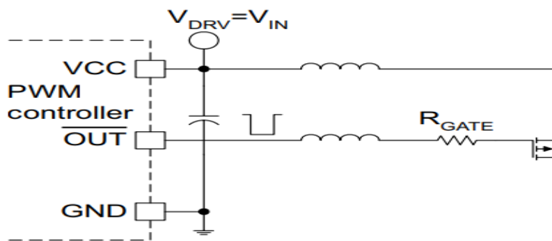
Figure I.32: Direct Drive for P-Channel MOSFET.[37]
