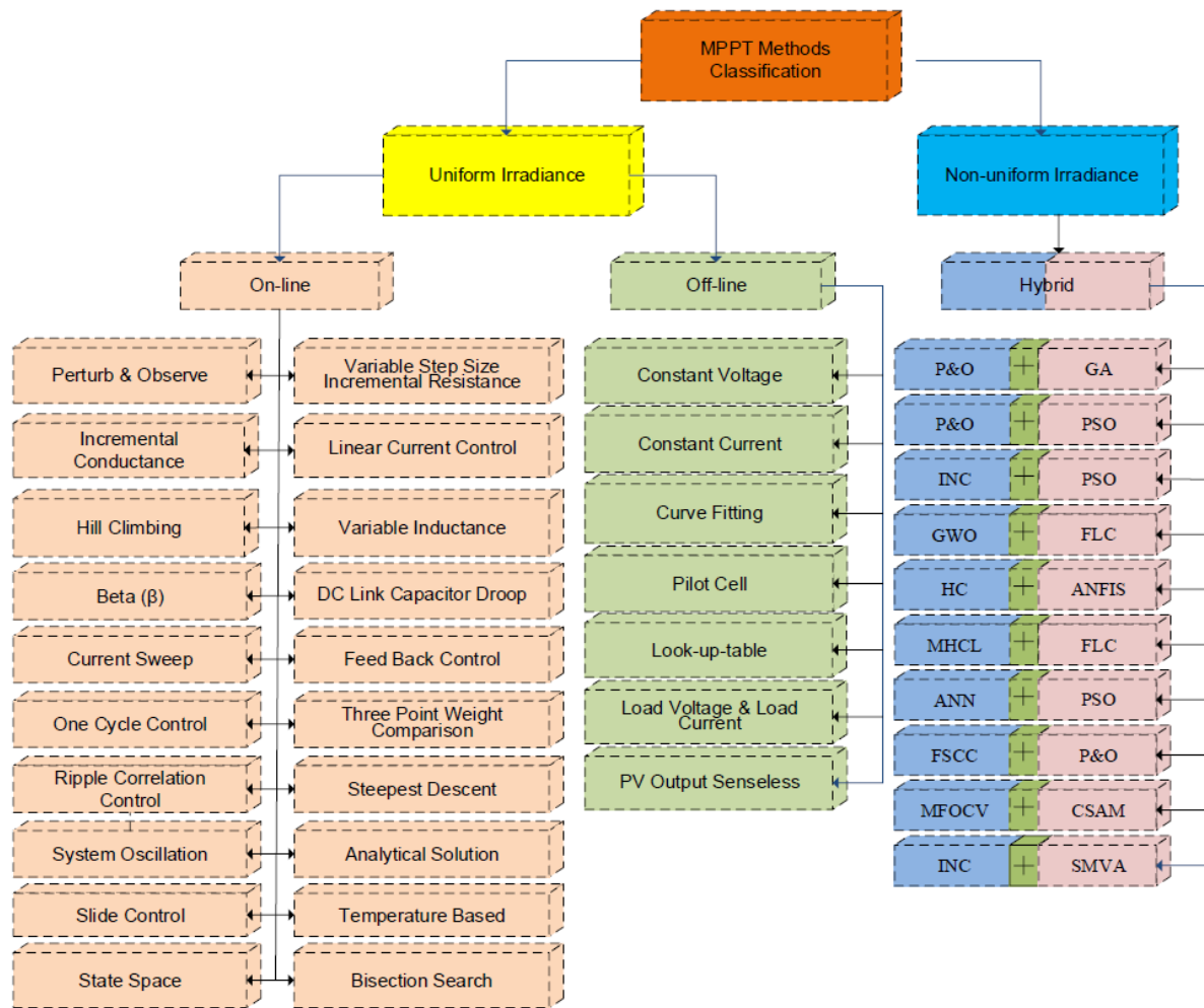
Figure II.5: MPPT Techniques Classification [62].
