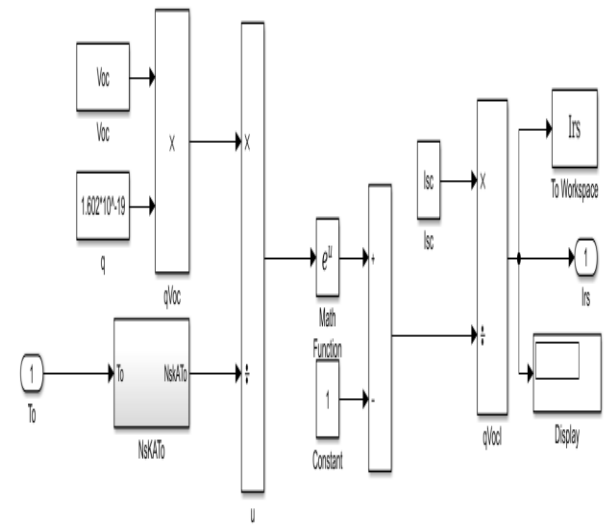
Figure II.12: Reverse saturation current model
