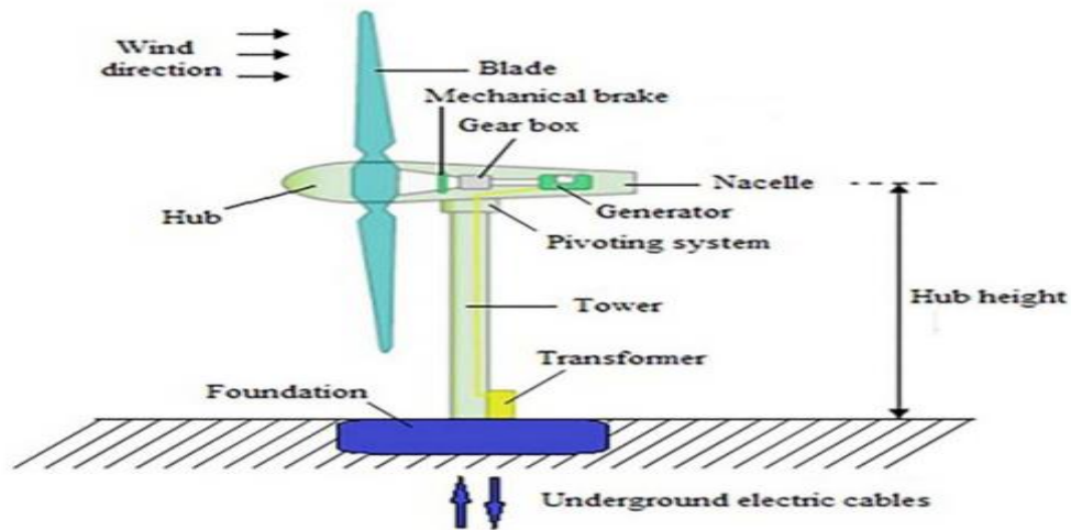
Figure I.9: Overview of main components for a wind turbine.[14]
