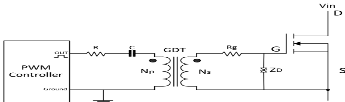
Figure I.34: Transformer insulated gate drive circuit diagram.[37]
