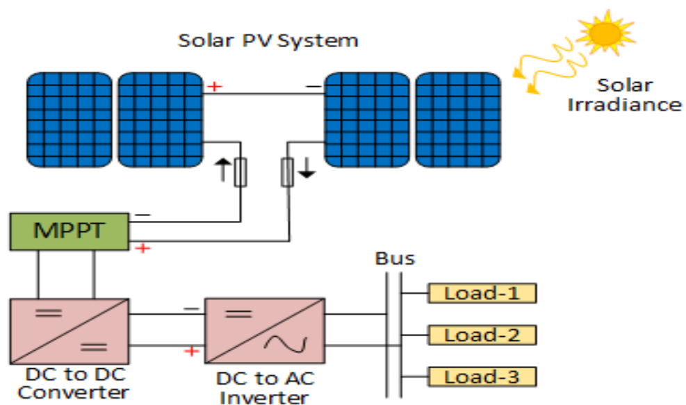
Figure II.1 Solar PV System with MPPT [57]
