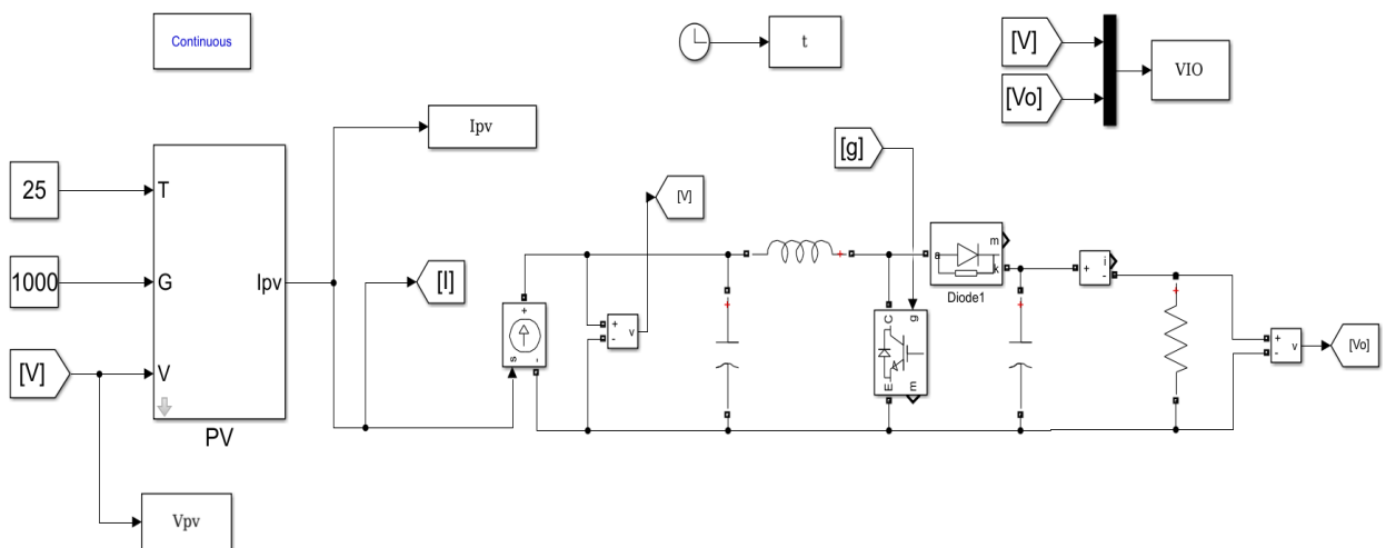
Figure II.20: Association of PV pannel with converter DC/DC boost
