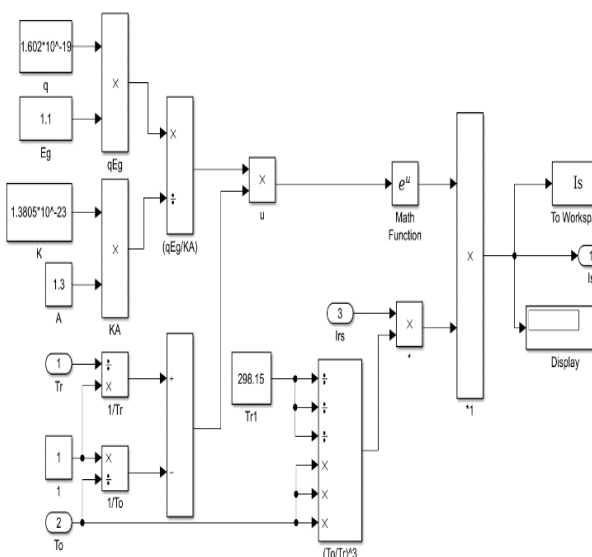
Figure II.13: saturation current model
