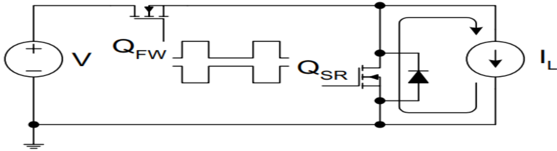
Figure I.31: Synchronous Rectification MOSFET Driver.[37]
