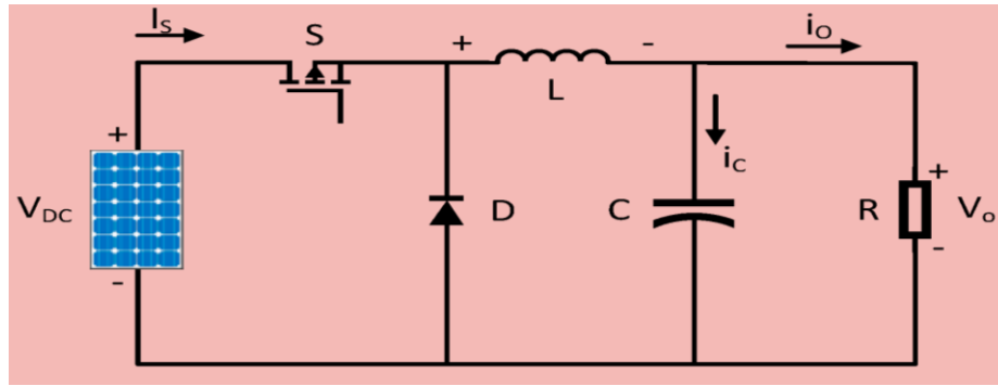
Figure II.3: Buck converter for the PV application [59].
