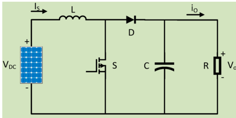
Figure II.2: Boost Converter for PV Application. [59]
