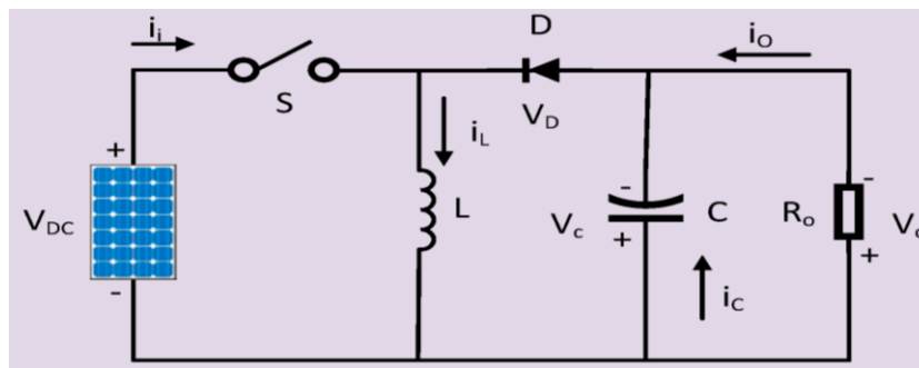
Figure II.4: Buck–Boost converter for PV application [59].
