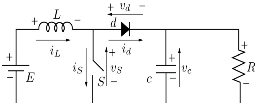
Figure II.17: Schematic representation of the DC-DC Boost converter [64].
