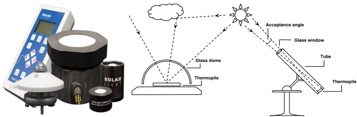
Figure I.39: A schematic illustration of a pyranometer and a pyrhelimeter.[42]
