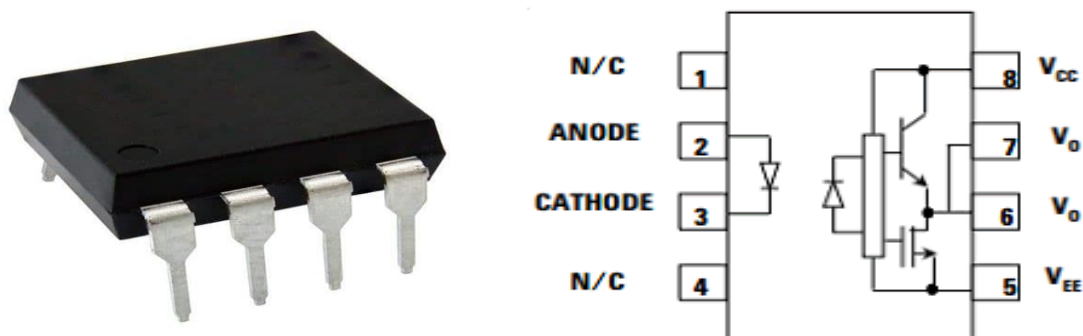
Figure.III.1 :Functional diagram.
