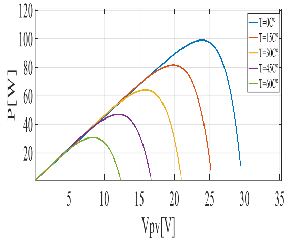
Figure II.27: Characteristics (P-V) for different temperature values at G= 1000\text{w/m}^2
