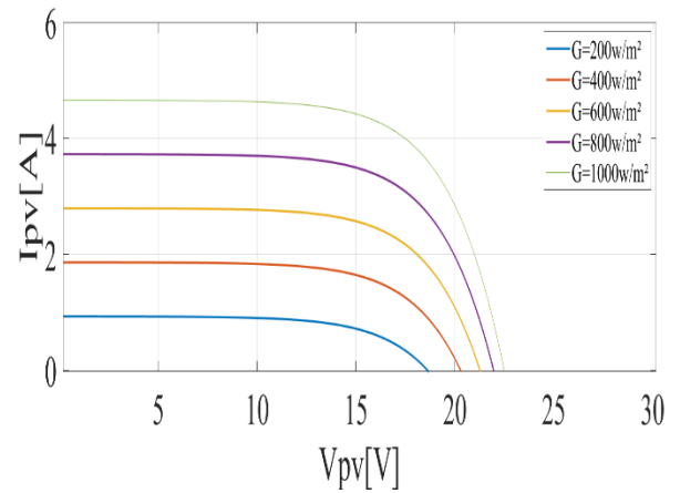
Figure II.38: Characteristics (I-V) for different radiation values at T= 25^{\circ}\text{C}
