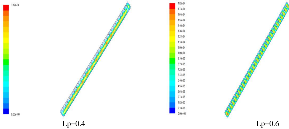
Figure 4. Stream lines for different values of L_p pour Ra=2.51 \cdot 10^4 , N=30 , \theta=45.0
