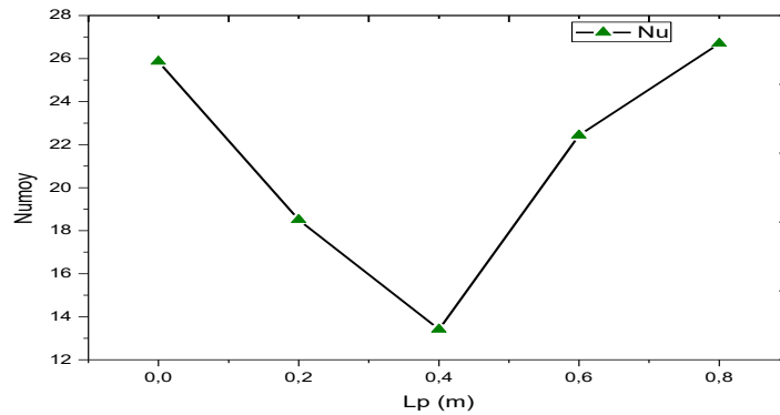
Figure 5. Variation in the number of average Nusselt for different values of L_p for Ra=2.51 \cdot 10^4 , N=30 , \varphi=45.0 .
