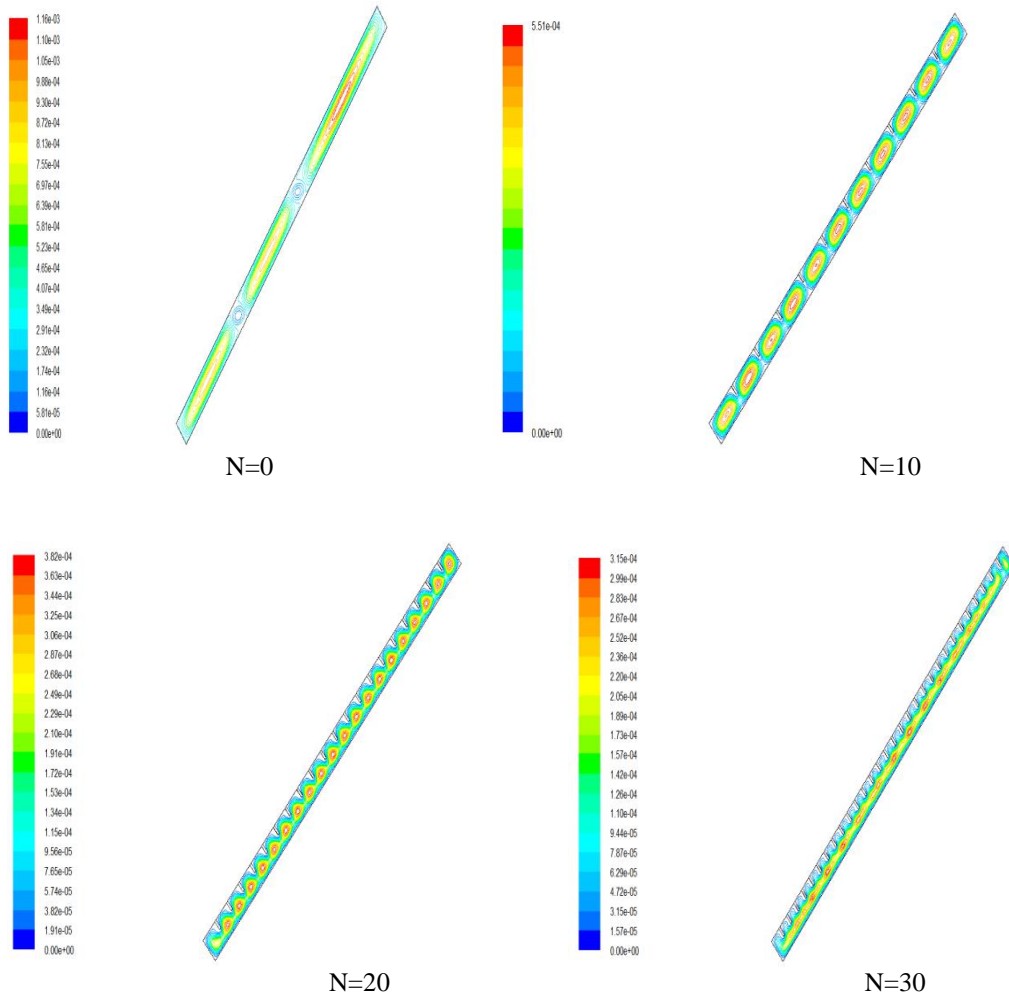
Figure 6. Streamlines for different values of the number of partitions N for Ra=2.51 \cdot 10^4 , Lp=0.4 , \varphi=45.0
