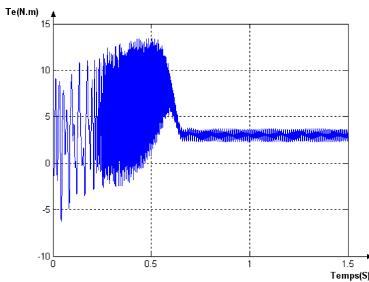
FigureIII.15.Variation du couple.
