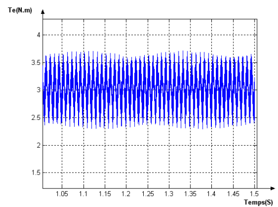
FigureIII.16.Variation du couple.
