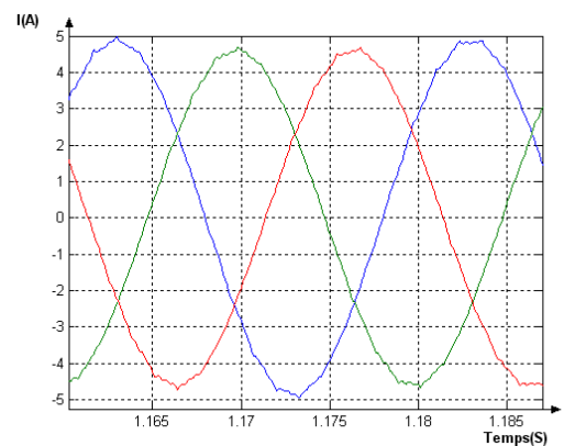
Figure III.10. Variation des courants.
