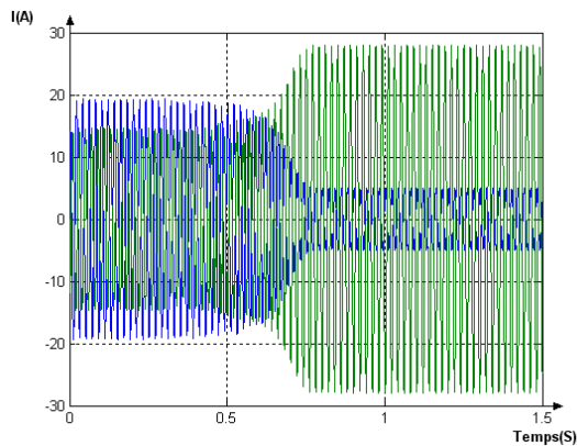
Figure III.9. Variation des courants.
