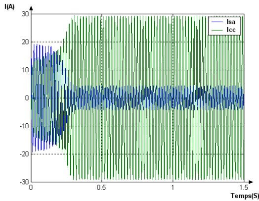
Figure III.2. Variation des courants.
