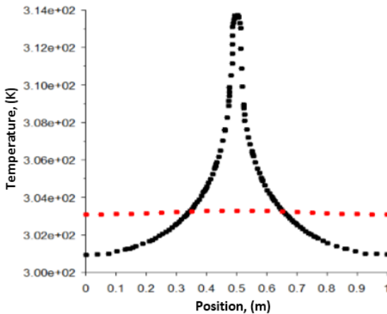
Figure 5.12 Temperature profile of one buried cable and the roadway under solar radiation
