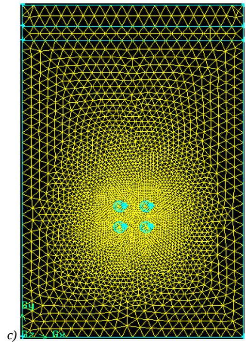
Fig. 2.3 Grid of computational domain a) single cable buried in soil, b) three buried cable, c) four buried cable
