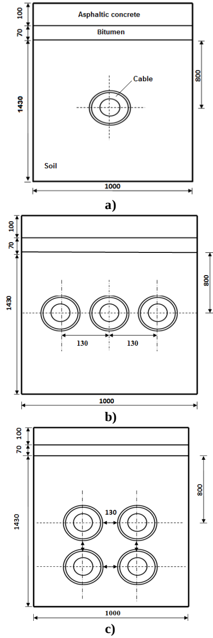
Fig. 2.2 Computational domain for numerical study a) of single copper cable buried in soil, b) three buried cable, c) four buried cable
