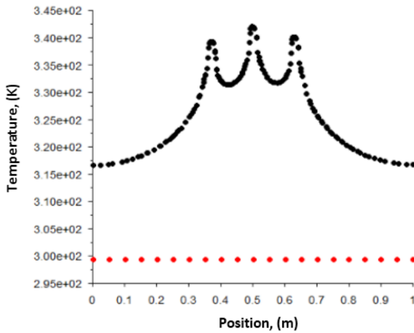
Figure 5.8 Average temperature profile at the three cable and the roadway
