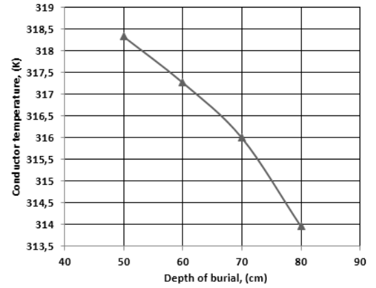
Fig. 5.2 Conductor temperature based on depth of burial
