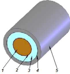
1. Copper conductor; 2. Conductor screen; 3. Insulation; 4. Copper screen; 5. Oversheath
