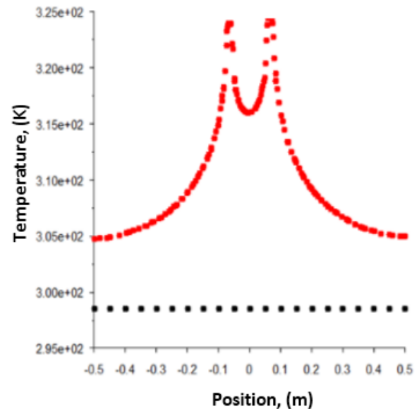
Fig. 5.10 Average temperature profile at the cables and the roadway
