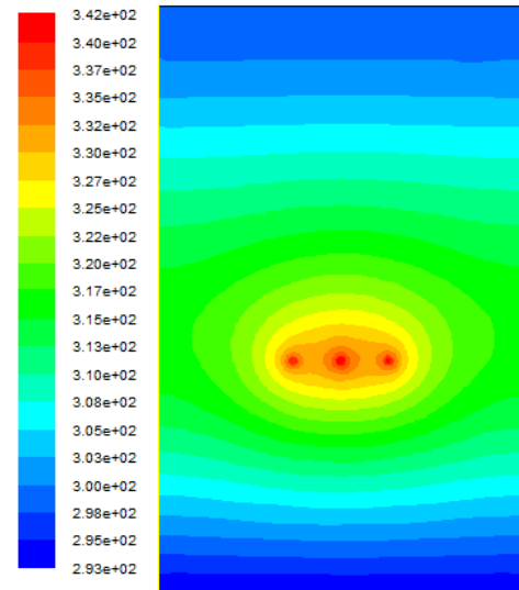
Fig. 5.7 Contours of temperature in a system of three buried cable
