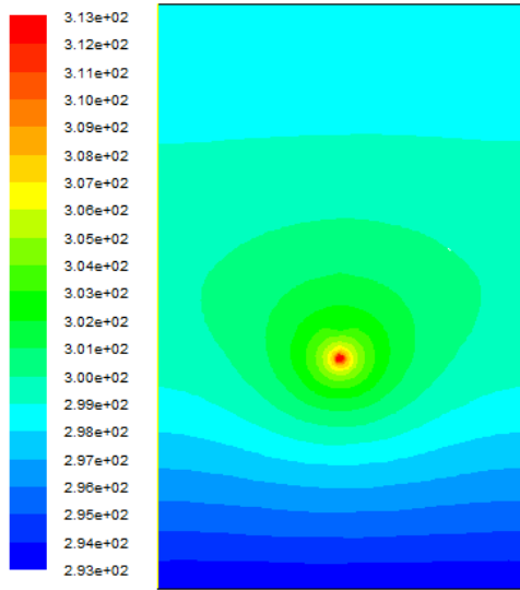
Fig. 5.5. Contours of temperature in a system of a single buried cable
