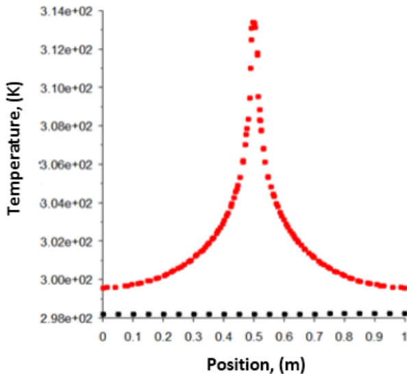
Fig. 5.6. Average temperature profile at the cable and the roadway
