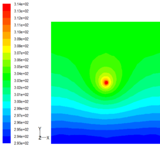
Fig. 5.11 Temperature contours of a cable under solar radiation
