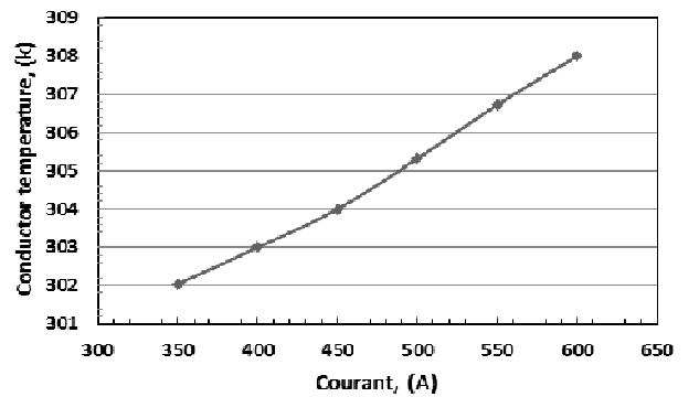
Fig. 5.4 Conductor temperature variation as a function of operating current
