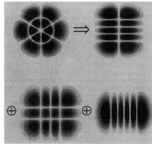
(b) The representation of an LG 13 LAGUERRE-GAUSSIAN mode from three HERMITE-GAUSSIAN modes TEM 14 , TEM 32 , and TEM 50 .
