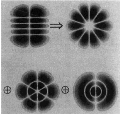
(a) The representation of a TEM 14 HERMITE-GAUSSIAN mode using three LAGUERRE-GAUSSIAN modes LG 05 , LG 13 , and LG 21 .
